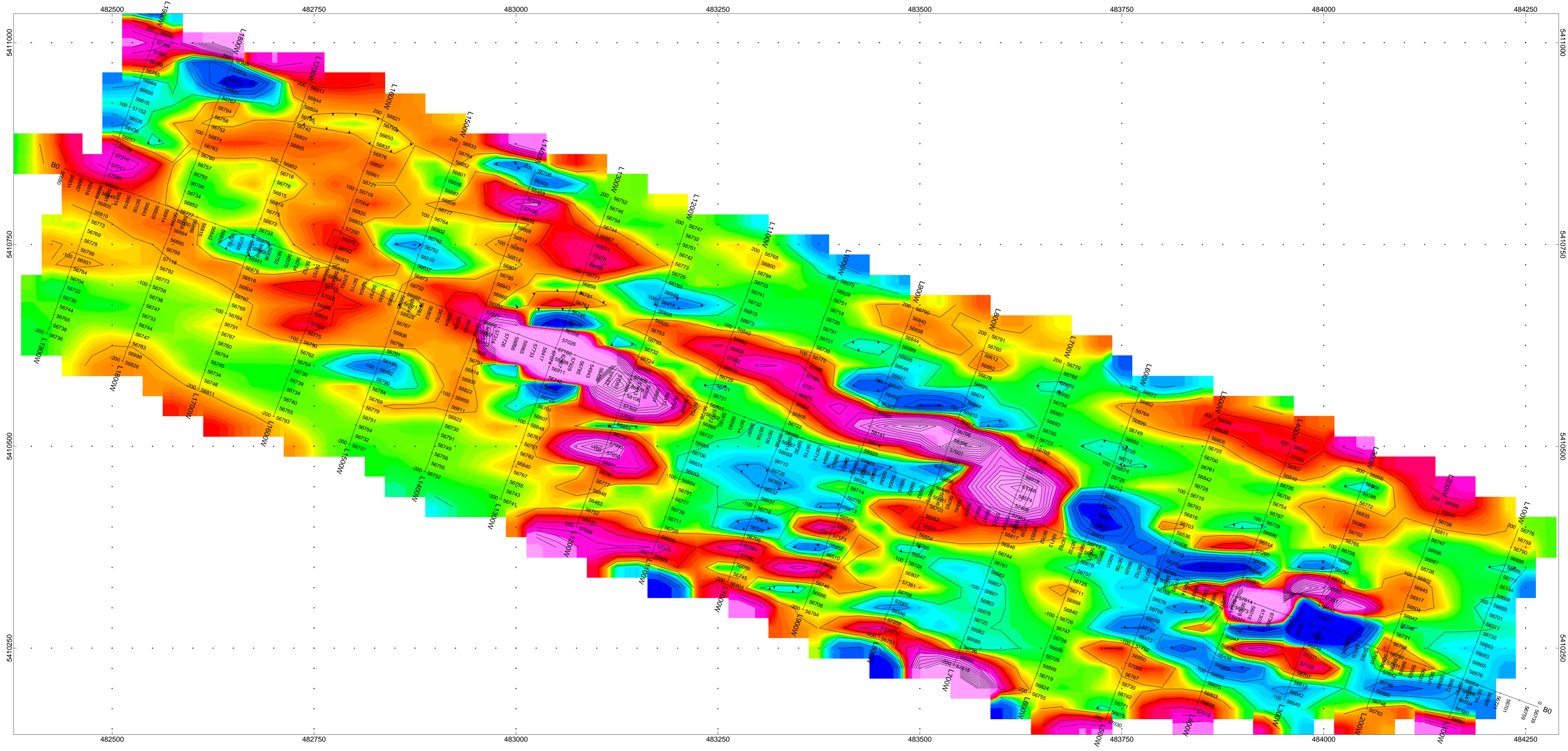
TOTAL FIELD MAGNETIC nanoTesla (nT)
